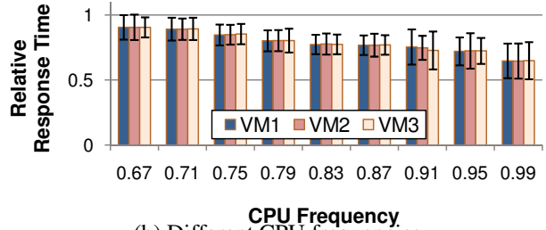
Figure 4. Performance of the load balancing controller under system model changes.
